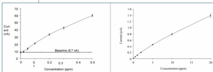
Figure 5. Free chlorine calibration curve; 'Low' range 0 to 0.5 ppm (mean RSD 3.8%), 'High' range free chlorine calibration curve from 0 to 20 ppm (mean RSD 4.2%).
