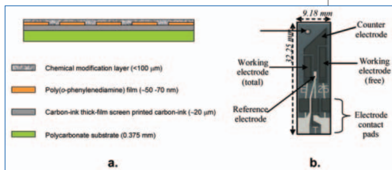
Figure 3. (a) Schematic of final sensor construction; (b) final four-electrode assembly.
