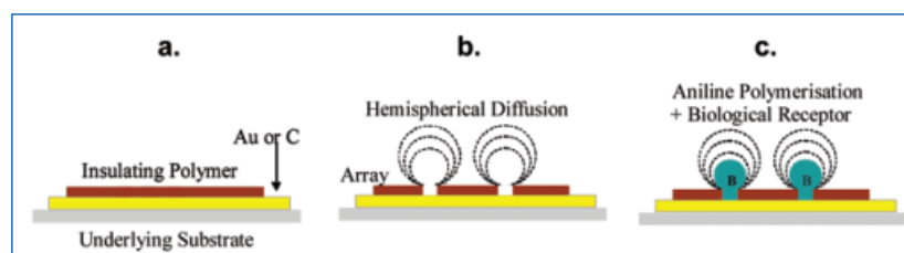
Figure 1. Schematic of formation of microelectrode arrays (a) deposition of insulating polymer, (b) sonochemical ablation to form microelectrodes, (c) deposition of polyaniline containing entrapped biological moieties.
