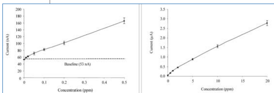
Figure 4. Combined chlorine calibration curve; 'Low' range from 0 to 0.5 ppm (mean RSD 4.1%), 'High' range from 0 to 20 ppm (mean RSD 4.3%).
