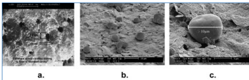
Figure 2. Scanning electron micrographs of (a) micropores formed by sonochemical ablation (b, c) polyaniline "mushrooms".
